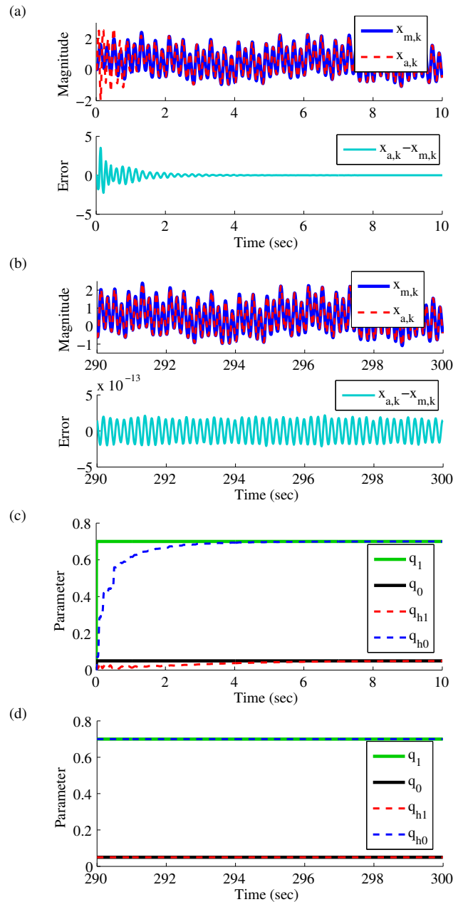
Fig. 3. Illustration of desirable dynamics tracking result when x_{r,k} = \frac{1}{2}(2 + \sin(0.4\pi kT) + \sin(2\pi kT) + \sin(5\pi kT) + \sin(10\pi kT) + \sin(20\pi kT)) and \theta_1 = 0.7, \theta_0 = 0.05 , (a) tracking result within 0 to 10 second period, (b) result within 290 to 300 second period, (c) parameters estimation result for the 0 to 10 second period, and (d) result for the 290 to 300 second period.
