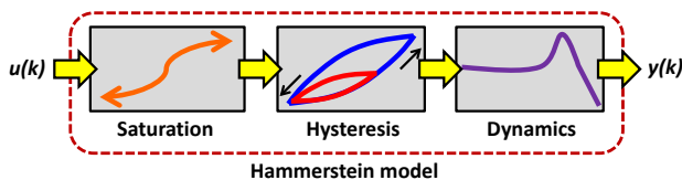
Fig. 1. Hammerstein model for smart material actuators considering saturation, hysteresis and dynamics characteristics.
