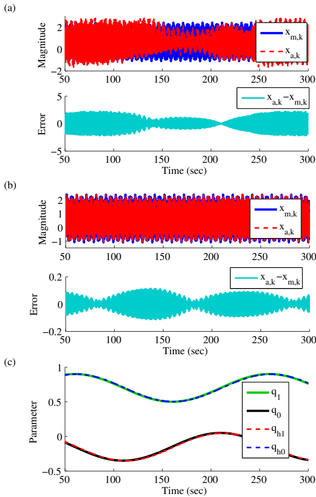
Fig. 4. Comparative test results of desirable dynamics tracking when \theta_1 = 0.7 + 0.2\sin(0.01\pi kT) and \theta_0 = -0.15 + 0.2\cos(0.01\pi kT) , (a) control result of plant with dynamic \theta_1, \theta_0 using controller with nominal \theta_1, \theta_0 , (b) result of plant with dynamic \theta_1, \theta_0 regulated by the proposed adaptive controller, and (c) estimation result of \theta_1, \theta_0 .
