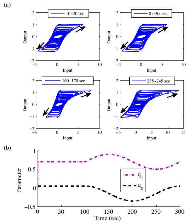
Fig. 2. Illustration of saturated hysteresis varying with parameter \theta_1 and \theta_0 , (a) input-output relation of saturated hysteresis, (b) saturation parameter \theta_0 and \theta_1 vary with time.
