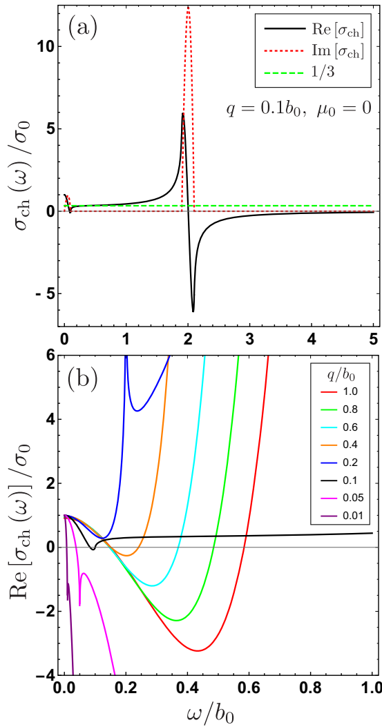
FIG. 2. The chiral magnetic conductivity as a function of frequency at zero temperature. (a) Real (black, solid) and imaginary (red, dotted) part of the chiral magnetic conductivity at q = 0.1b_0 , \mu_0 = 0 . The green dashed line indicates 1/3 . (b) The real part of the chiral magnetic conductivity for a set of values q . All the conductivities are scaled by \sigma_0 = e^2 b_0 / 2\pi^2 .
