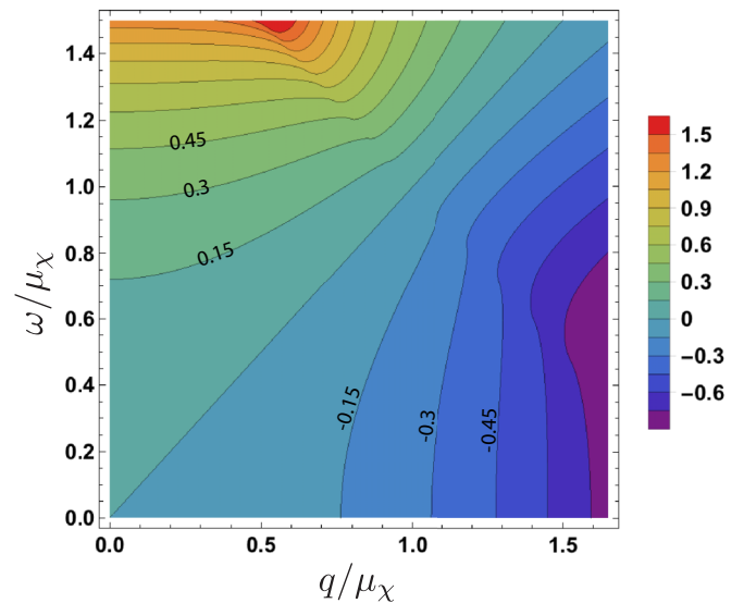
FIG. 3. Contour plot of the difference between the real part of the chiral magnetic conductivity of one Weyl node in Eq. (61) and that of Eq. (84) in Ref. [22] at zero temperature. The results are normalized to e^2 \mu_\chi / 12\pi^2 .
