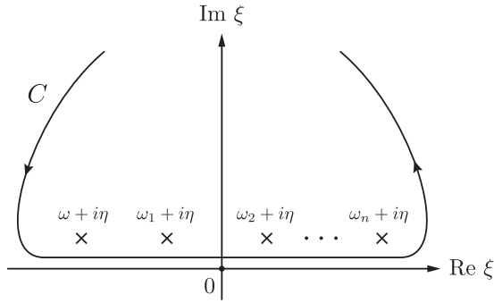
FIG. 4. Contour in the upper half \xi plane for Cauchy integral with n + 1 poles in Eq. (E1).
