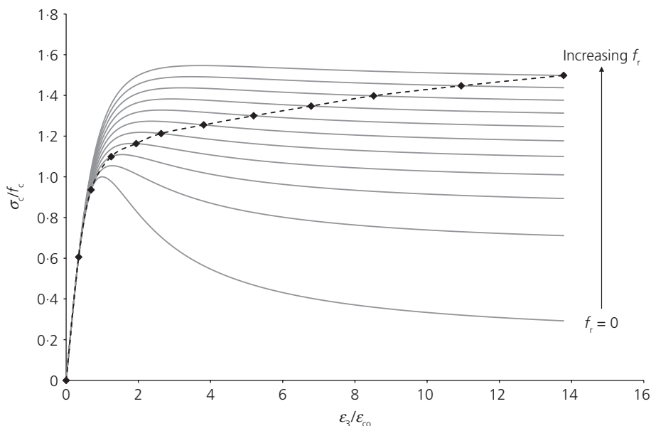
Figure 3. Typical compressive stress–strain relation of FRP-confined concrete
