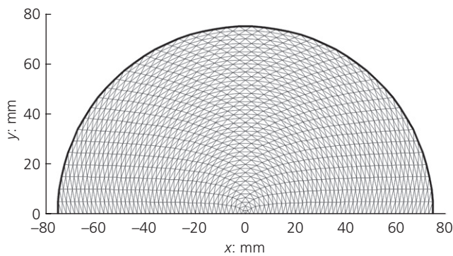
Figure 6. 2D mesh of a FRP-confined circular concrete column section
