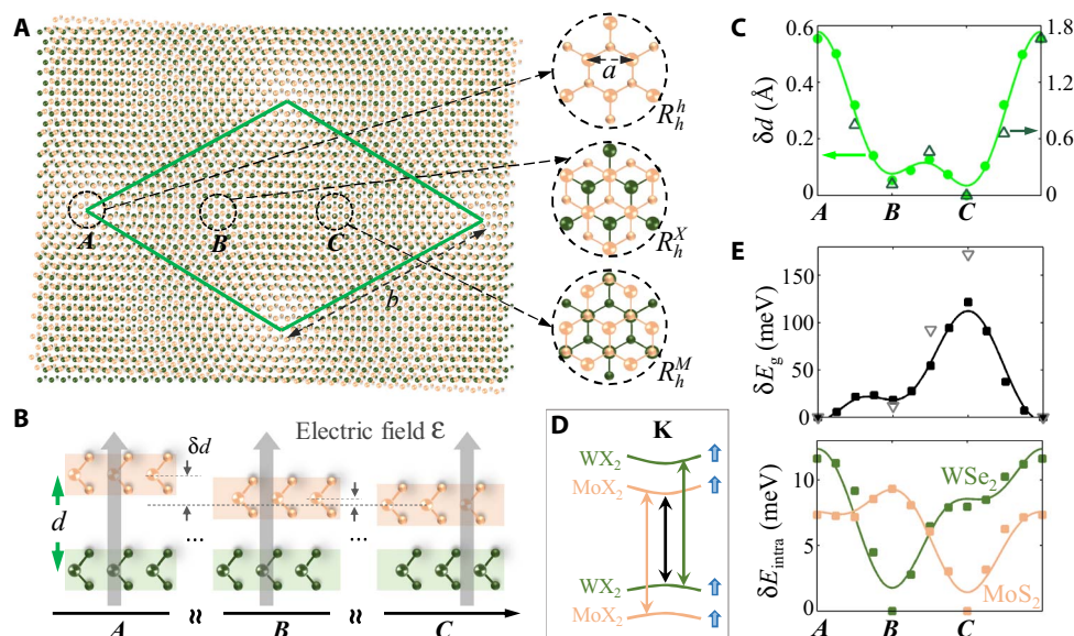
Fig. 1. Moiré modulated local energy gaps and topographic height in the heterobilayer. (A) Long-period moiré pattern in an \text{MoX}_2/\text{WX}_2 heterobilayer. Green diamond is a supercell. Insets are close-ups of three locals, where atomic registries resemble lattice-matched bilayers of different R-type stacking. (B and C) Dependence of interlayer distance d on the atomic registries. In (C), dots are our first-principles calculations for the \text{MoS}_2/\text{WSe}_2 heterobilayer, and triangles are the scanning tunneling microscopy (STM) measured variation of the local d values in a b = 8.7 nm \text{MoS}_2/\text{WSe}_2 moiré in the study of Zhang et al. (26). The variation in d then leads to laterally modulated interlayer bias ( \propto d ) in a uniform perpendicular electric field, as (B) illustrates. (D) Schematic of relevant heterobilayer bands at the \mathbf{K} valley, predominantly localized in either the \text{MoX}_2 or \text{WX}_2 layer. (E) Top: Variation of the local bandgap E_g [black arrow in (D)] in the \text{MoS}_2/\text{WSe}_2 moiré. Bottom: Variation of the local intralayer gaps [denoted by arrows of the same color in (D)]. In (C) and (E), the horizontal axis corresponds to the long diagonal of the moiré supercell, and the vertical axis plots the differences of the quantities from their minimal values. The curves are fitting of the data points using eqs. S2 and S3 in section S1.
