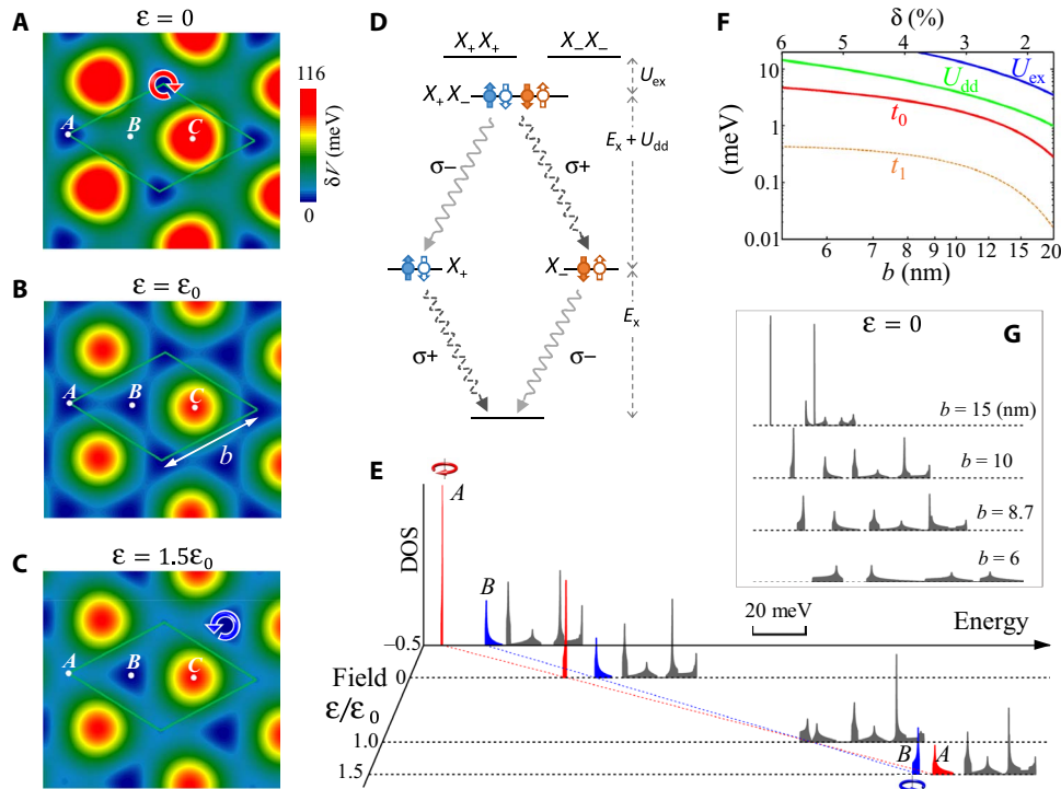
Fig. 3. Electrically tunable and strain-tunable quantum emitter arrays. (A to C) Tuning of excitonic potential by perpendicular electric field ( \epsilon ) in the R-type \text{MoS}_2/\text{WSe}_2 moiré. At zero field, nanodot confinements are at A points, realizing periodic array of excitonic quantum emitters, which are switched to B points at moderate field (see the main text). (D) Spin optical selection rule of quantum emitter at A . When loaded with two excitons, the cascaded emission generates a polarization-entangled photon pair. The optical selection rule is inverted when the quantum emitter is shifted to B [see (A) and (C)]. (E) Electric field tuning of exciton density of states (DOS) in the R-type \text{MoS}_2/\text{WSe}_2 moiré with b = 10 nm. The field dependence of V(\mathbf{A}) and V(\mathbf{B}) are denoted by the dotted blue and red lines on the field-energy plane. The colors of the two lowest energy peaks distinguish their different orbital compositions at A and B points in the moiré. (F) Exciton hopping integral between nearest-neighbor (NN) A and B dots in (B) ( t_0 ), between NN A dots ( t_1 ), and on-site exciton dipole-dipole ( U_{dd} ) and exchange ( U_{ex} ) interactions as functions of the moiré period b (see sections S4 and S5). The top horizontal axis is the corresponding lattice mismatch \delta for rotationally aligned bilayer. (G) Exciton DOS at different b at zero electric field. The 20-meV scale bar applies for the energy axis in (E) and (G).
