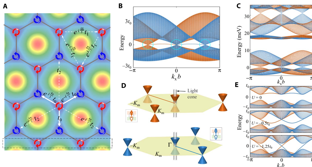
Fig. 4. Spin-orbit-coupled honeycomb lattices and Weyl nodes. (A) Opposite photon emission polarization at A and B sites and complex hopping matrix elements for the spin-up exciton. (B) Exciton spectrum at V(\mathbf{A}) = V(\mathbf{B}) and moiré period b = 10 nm, from the tight-binding model with the third NN hopping. t_0 = 2.11 meV, t_1 = 0.25 meV, and t_2 = 0.14 meV. The bands feature a Dirac node and two Weyl nodes (highlighted by dotted circles). These magnetic monopoles are linked by an edge mode at a zigzag boundary, with spin polarization reversal at the Dirac node. Spin-down (spin-up) exciton is denoted by brown (blue) color. (C) Exact exciton spectrum in this superlattice potential (see section S4). Dirac/Weyl nodes are also seen in higher energy bands. (D) Schematic of the Dirac cones for the spin-up and spin-down excitons in the moiré-Brillouin zone (m-BZ), and edge modes at a zigzag boundary. Exciton-photon interconversion can directly happen within the shown light cone. (E) The Dirac and Weyl nodes are gapped by a finite A-B site energy difference \Delta = 0.5t_0 , whereas the edge band dispersion is tuned by changing the on-site energy of the dots on the zigzag boundary [enclosed by the dashed box in (A)] by the amount U .
