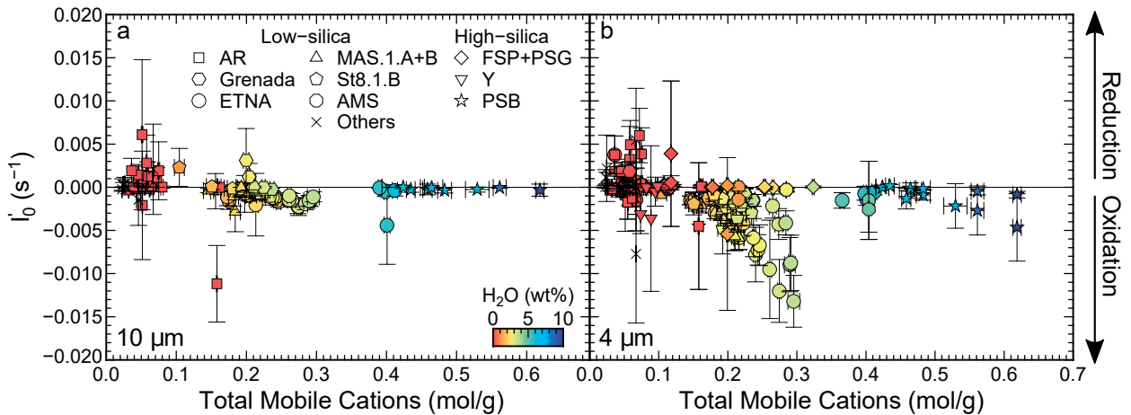
FIGURE 8. The rate of change of FeL\beta\gamma/FeL\alpha\tau with time at time zero ( I'_0 ) against Total Mobile Cations (TMC, molar sum of H_2O+Na_2O+K_2O per gram of glass), where symbol shape indicates average glass composition (Table 1) and color indicates H_2O . Analytical conditions were: 15 kV accelerating voltage, 50 nA beam current, and (a) 10 and (b) 4 \mu m beam diameter.
