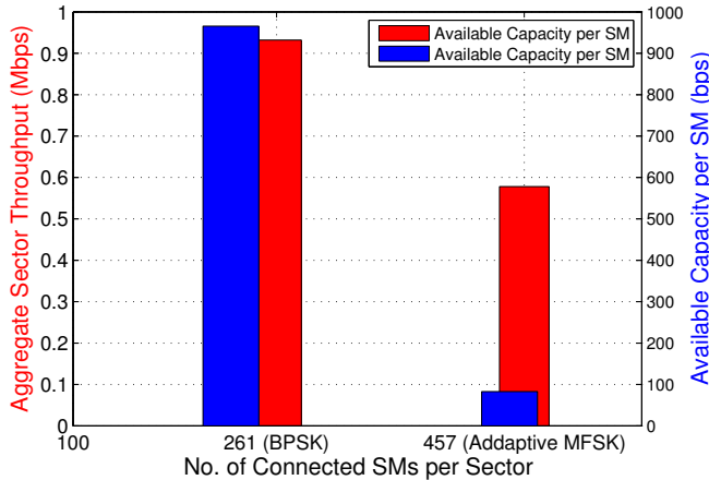
Fig. 11: Capacity analysis for the uplink rural case with R=4\text{Km} .
