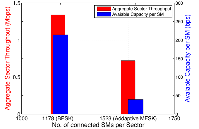
Fig. 10: Capacity analysis for the sector urban case with R=0.5\text{Km} .
