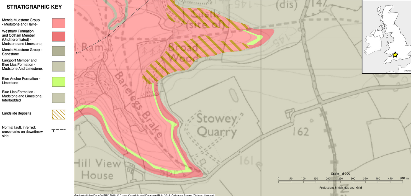
Fig. 2. Geology around Stowey Quarry (ST 597586). The morphological top of Sutton Hill is dominated by Early Jurassic outcrops, but the Penarth Group strata are buried just a few metres below the ground in Stowey Quarry and crop out on the plateau's slopes. Stowey Quarry was opened to work the Early Jurassic rocks, and the floor rested on the Rhaetian-Lias contact. © Crown Copyright and Database Right 2015. Ordnance Survey (Digimap License).
