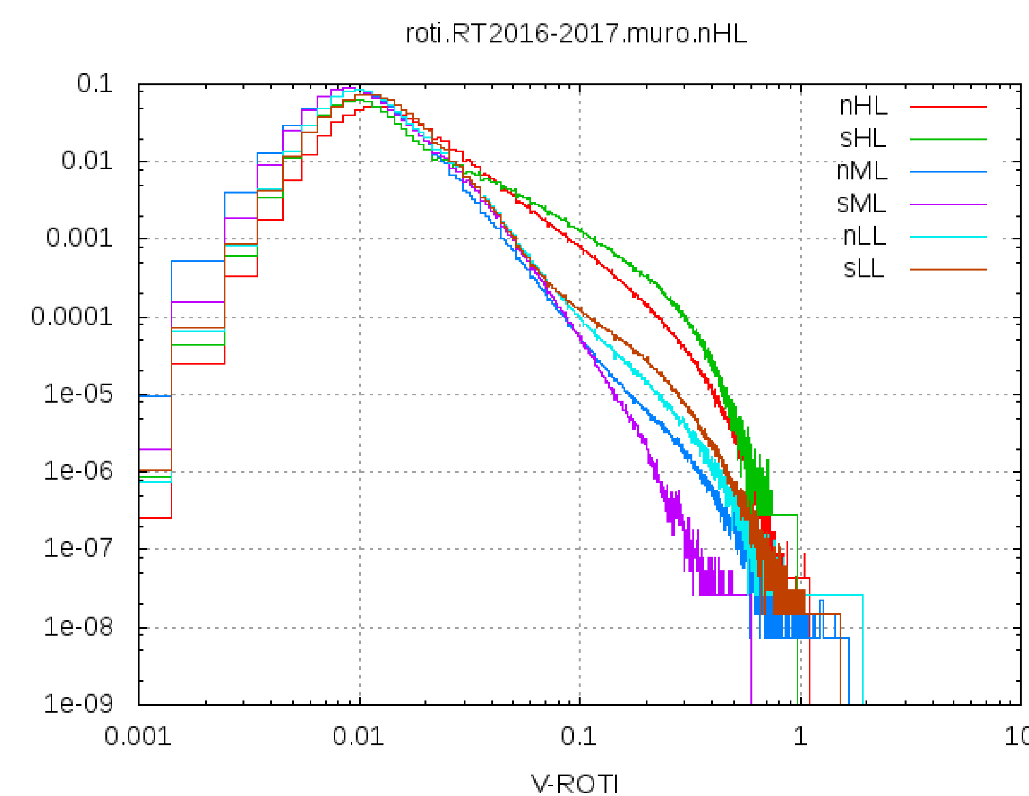
Log-log histograms of ROTI occurrence for xYL (x = n,s for north,south, Y=H,M,L for high, mid., low latitudes)
