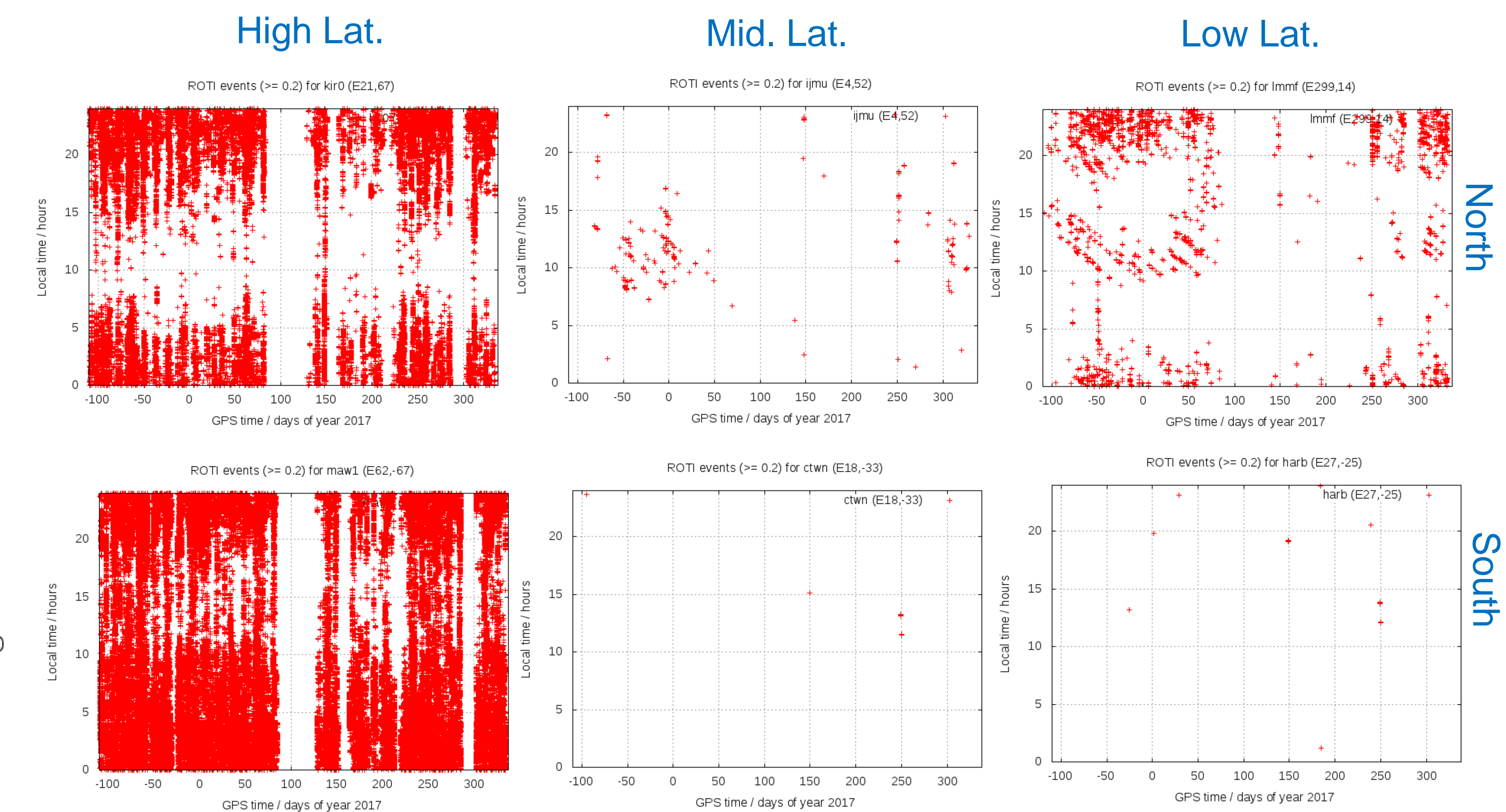
RT-ROTI events in LT vs time for the six 30°-latitudinal strips
