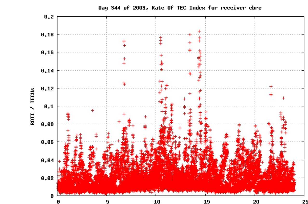
Example of ROTI evolution for IGS receiver EBRE during the day 344 of 2003
