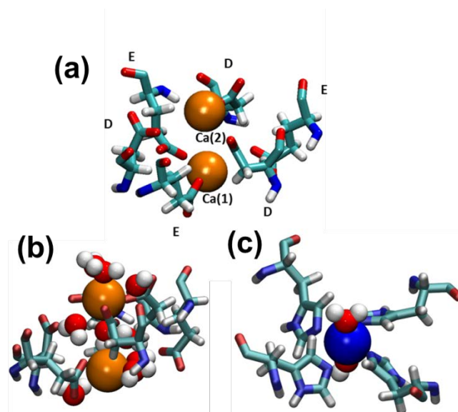
Fig. 2 (a) Averaged structure of C 3 pore interface. The metal ions and their coordination sphere are shown. E and D refer to Asp and Glu residues, respectively. Details about the metal coordination with protein residues and water molecules for the (b) C 3 and (c) C 4 pore interfaces are also shown. All figures were extracted from the simulation of the whole Cu-cage system.
