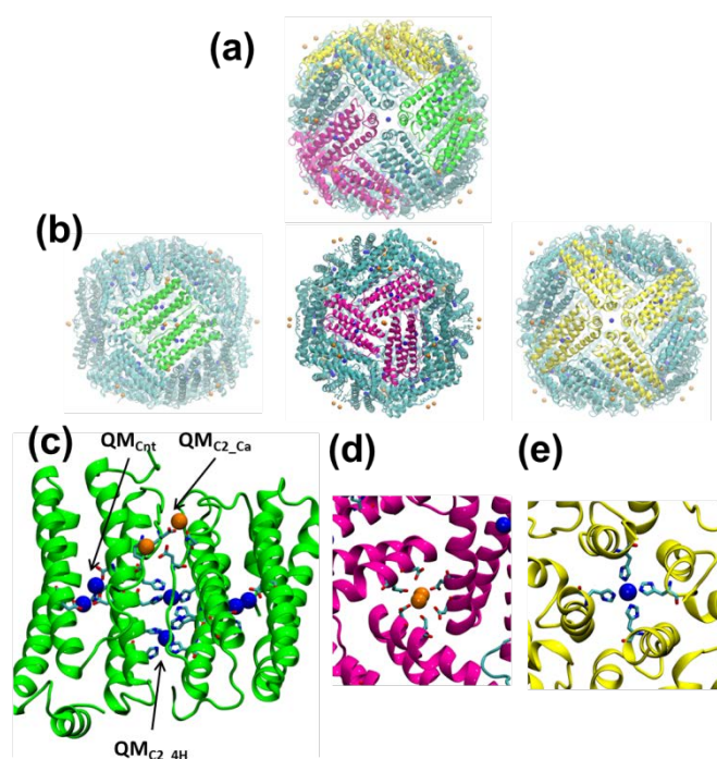
Fig. 1 (a) Top view of the Cu-4His- \Delta C^* cage. (b) Alternative views of Cu-4His- \Delta C^* cage: C_4 pore interface view through the C_2 symmetry axis (left); C_3 pore interface view through the C_3 symmetry axis (middle); and C_2 pore interface view through the C_4 symmetry axis (right). (c) General view of the quantum regions in the C_2 dimer interface. Details of the two Cu^{2+} coordination sites through His residues ( QM_{C_2,4H} ), the two Ca^{2+} coordination sites ( QM_{C_2,Ca} ), and the two Cu^{2+} coordination sites in the centre of the monomer ( QM_{Cnt} ). (d) Detail of the quantum region in the C_3 pore interface and (e) C_4 pore interface in Cu-cage. The C_2 , C_3 and C_4 pore interfaces are highlighted in green, pink and yellow, respectively. The transition metal ( Cu^{2+} or Ni^{2+} ) and the Ca^{2+} ions are highlighted in blue and orange, respectively.
