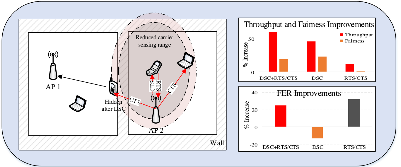
Fig. 4: TGax proposal for CCA modification and controlled use of RTS/CTS mechanisms.
