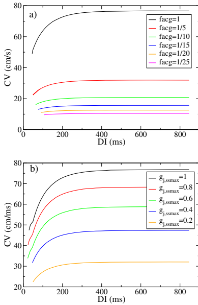
Figure 2. Curves of velocity restitution corresponding to a fiber with homotypic-homomeric connexin Cx43 gap junctions for different a) g_{j,ss} multiplying factors and b) maximum conductivity g_{j,max} values.
