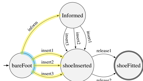
Fig. 1: Graphical example of decision-making (blue) and configuration preferences (yellow): in this action-sequence flow for the shoe fitting task, represented as a FSA, decision-making preferences aid to choose among alternative paths, while the configuration ones help to tune action parameters.
