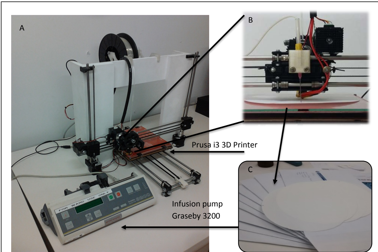
Figure 1 (a) Schematic of the one-step plotting method for patterning paper with the use of a Prusa i3 printer and an infusion pump Graseby 3200. (b) Detail of the needle adaptor at the Prusa i3. (c) Photo of a manufactured sisal paper.
