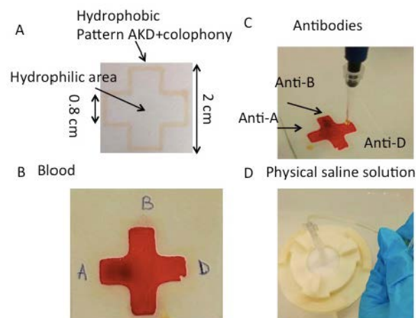
Figure 4 (a) Hydrophobic pattern for ABO blood typing (b) Blood sample deposition (c) Antibodies deposition (d) Washing step with saline solution
