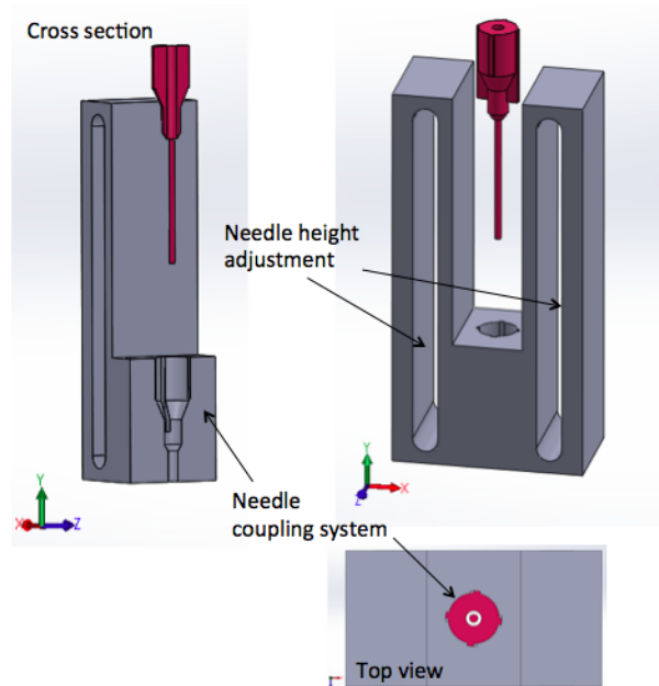
Figure 2 -3d printed part to position the ink injector.
