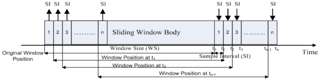
Fig. 2. Sliding Window Algorithm
