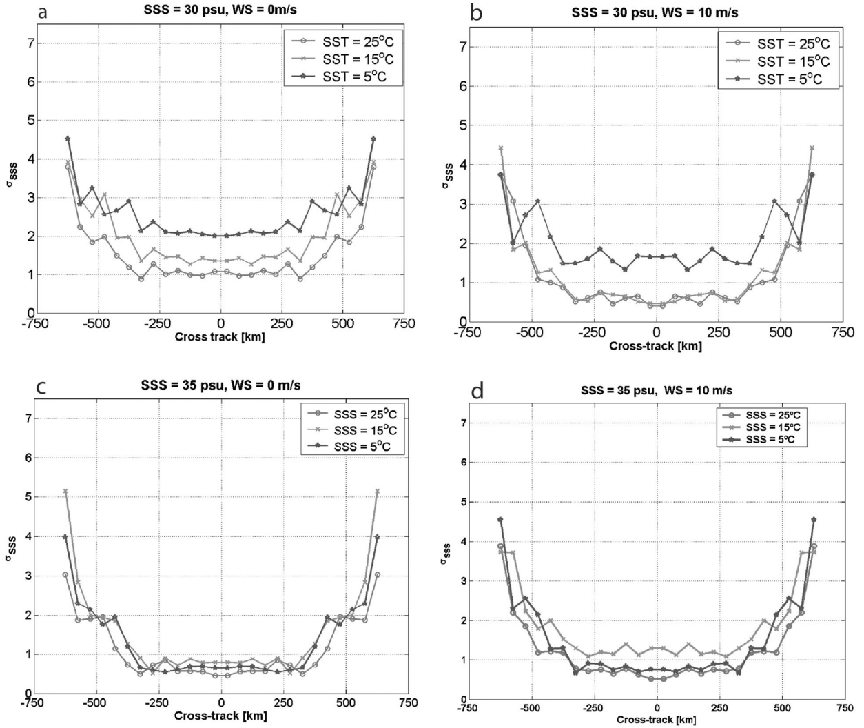
Figure 5. Simulated standard deviation of the retrieved SSS for different wind speed 0 m/s (left) and 10 m/s (right), different SSS (a and b) 30 psu, (c and d) 35 psu and (e and f) 40 psu, and different SST: 5°C (stars), 15°C (crosses) and 25°C (circles). See color version of this figure at the back of this issue.
