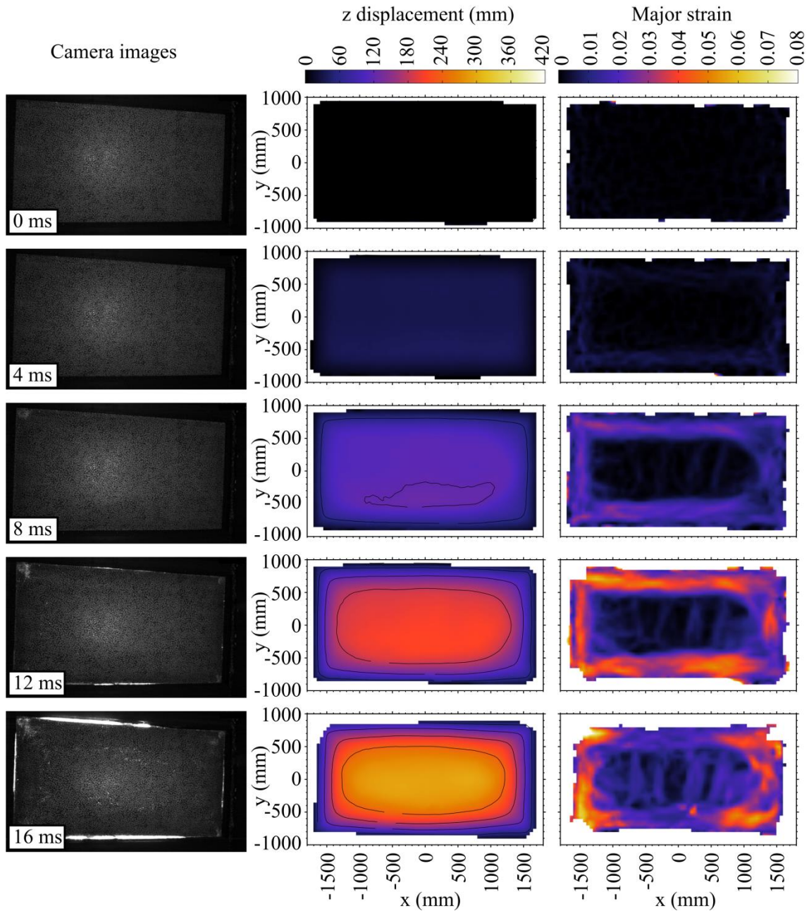
Figure 7: DIC results for Test 4.
