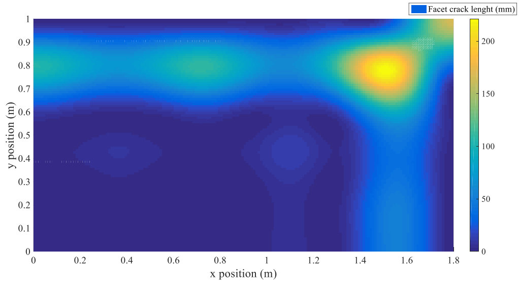
Figure 9: Test 4 estimated crack spacing at 1.5 ms.
