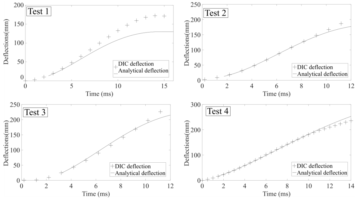
Figure 13: Calculated and experimental central deflection for Tests 1 to 4.
