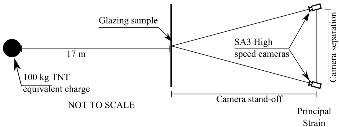
Figure 3: Typical test and DIC set up (adapted from [25]).
