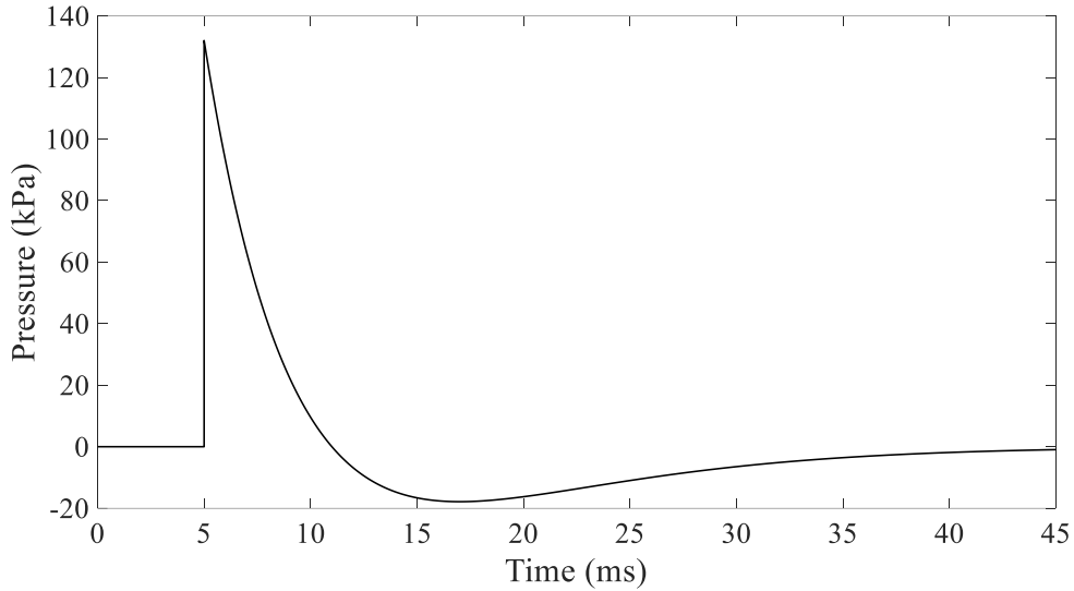
Figure 4: Plot of the function used to represent the blast pressure.
