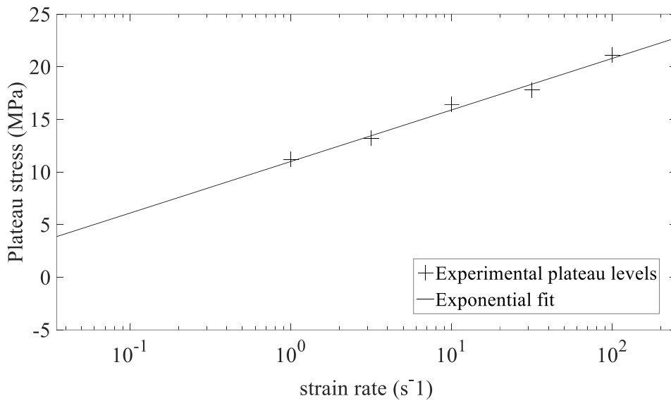
Figure 5: Crazed glass plateau stresses plotted against the strain rate. Hooper's [27] logarithmic fit is also shown.
