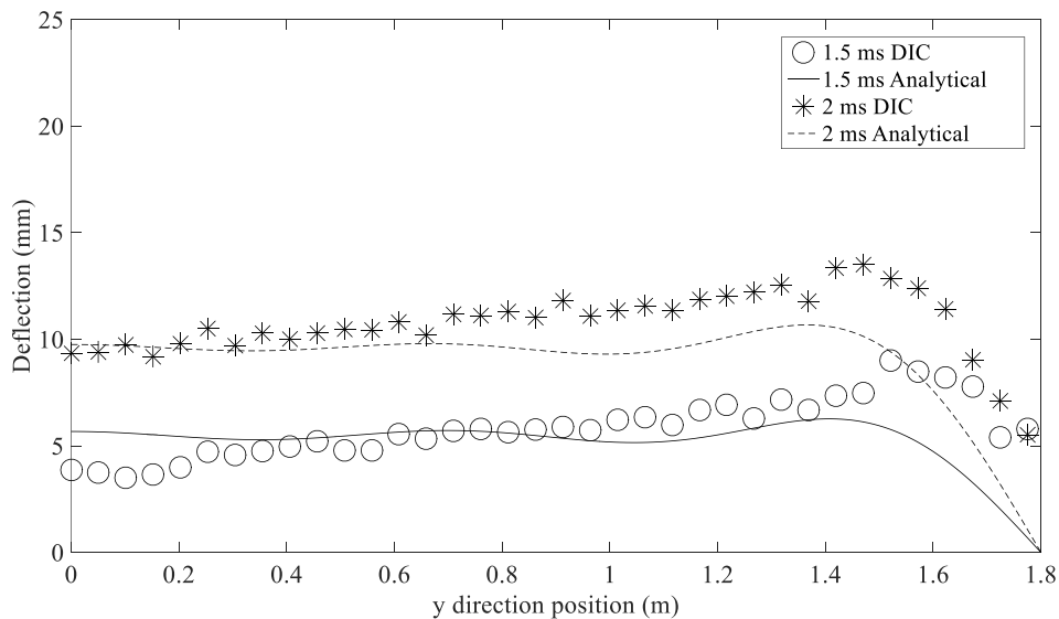
Figure 8: Test 4 pre-crack deflection along a centre line cut across the pane. Two time points are shown for clarity.
