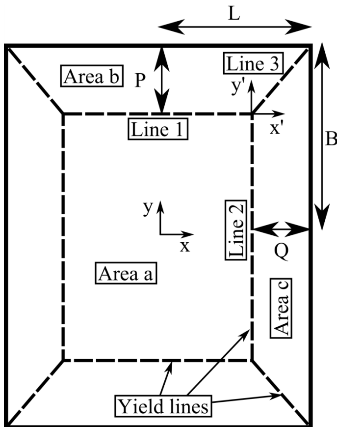
Figure 6: Typical location of the yield lines assumed in the system.
