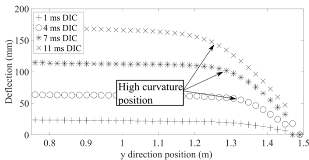
Figure 1: Deformation along a centre line of the window in Test 3 (adapted from [4]).
