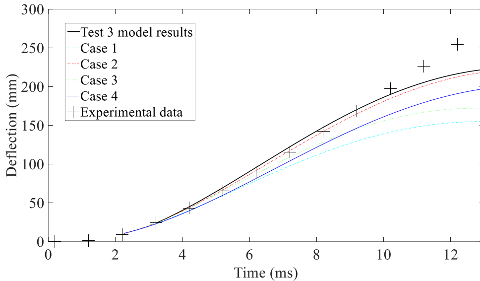
Figure 15: Central out of plane deflection for the cases run as part of the sensitivity analysis on the blast pulse parameters.
