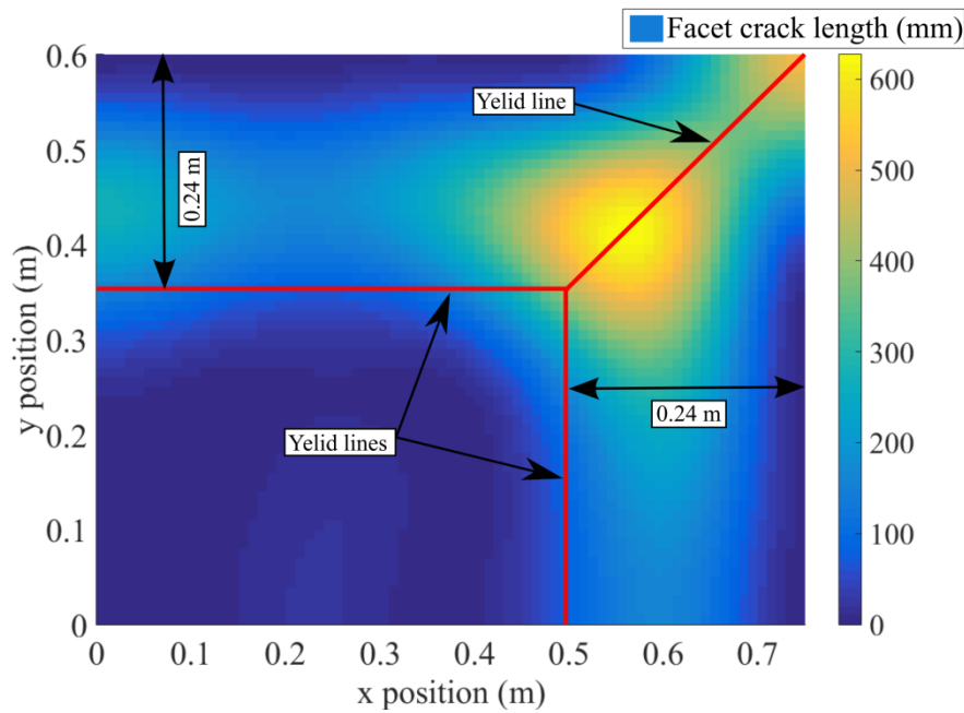
Figure 10: Yield line position in Test 3. The position is superimposed to the crack spacing results plot.
