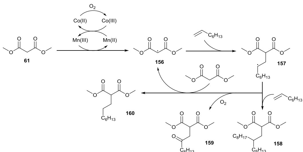
Scheme 53 Catalytic radical addition of carbonyl compounds to alkenes by \text{Mn(II)/Co(II)/O}_2
