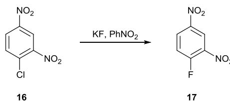
Scheme 4 Nucleophilic halogen exchange used in fluoroarene synthesis
