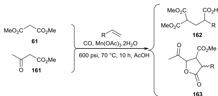
Scheme 55 Products obtained from ketoesters or malonates with \text{Mn}(\text{OAc})_3/\text{CO}
