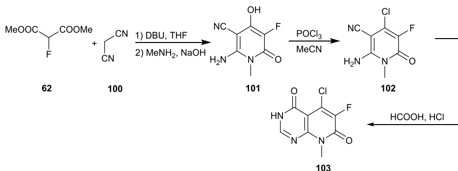
Scheme 35 Synthesis of 6-fluoro-8-methylpyrido[2,3-d]pyrimidine-4,7-(3H,8H)-dione
