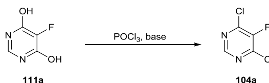
Scheme 43 Chlorination of 4,6-dihydroxy-5-fluoropyrimidine 111a using \text{POCl}_3
