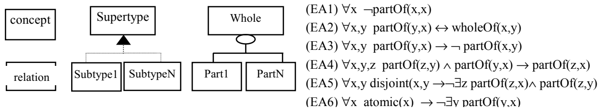
Figure 3. LINGO's notation [7].
