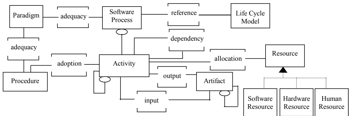
Figure 2. Software process ontology [16].
