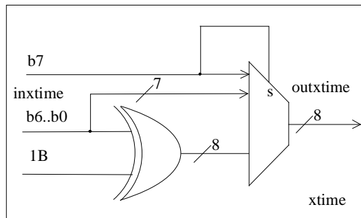
Figure 7 – Xtime Operation
