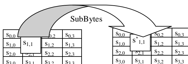
Figure 2 – SubBytes Transformation
