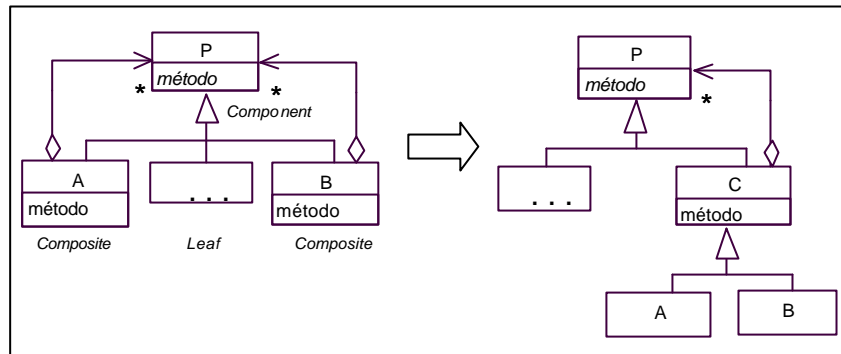
Figura 2: Refactoring Extract Composite
