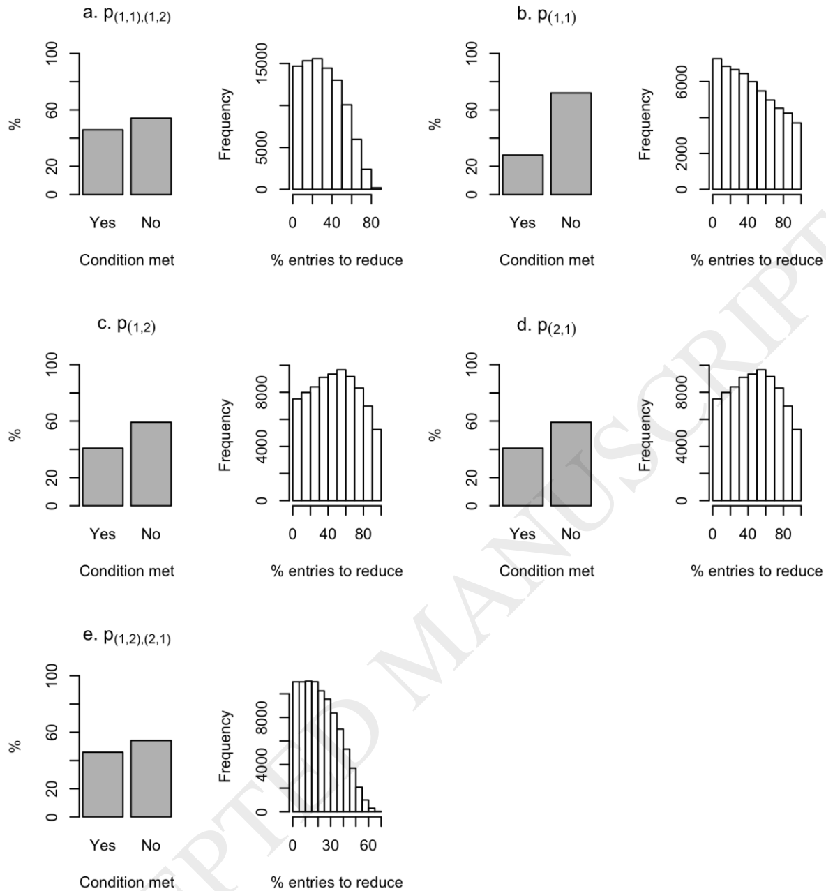
Figure 5: Percentage of the 2 \times 10^5 LH samples for which the conditions identified in Table 2 were met for the target reproduction number and corresponding percentage of S entries that need to be reduced to eradicate infection via rodent control a) all transmission routes can exist, b) only vertical and direct transmission exist, and for environmental control c) only environmental transmission exists, d) environmental transmission exists, and e) no constraints on which infection routes exist.
