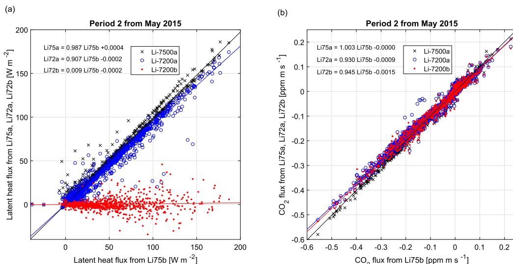
FIG. 4. A comparison of measured (a) latent heat flux and (b) CO_2 flux between the Li75b instrument and the other three instruments for period 2 when a Nafion dryer was installed on one of the Li-Cor 7200 instruments (Li72b). A comparison of the two Li-7500 instruments is shown (black crosses). A comparison of fluxes between the undried Li-7200 without a mounted Nafion dryer and one of the Li-7500 instruments is shown (blue circles). A comparison of the CO_2 fluxes with the dried Li-7200 to the same Li-7500 (red dots). Three fitted lines are included with the data in the corresponding color scheme, and the fitted expressions are given in the upper left of each plot.
