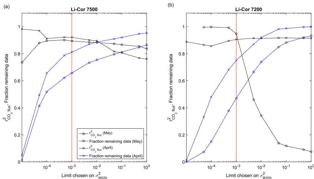
FIG. 3. The squared correlation coefficient for the \text{CO}_2 flux ( r_{\text{CO}_2}^2 , black), and the fraction of remaining data (blue) is shown as a function of different threshold limits for the variance of the RSSI value ( \sigma_{\text{RSSI}}^2 ). The result for the (a) two Li-Cor 7500 instruments and (b) two Li-Cor 7200 instruments. Data from April 2015 (lines with crosses) and May 2015 (lines with circles). The threshold limit \sigma_{\text{RSSI}}^2 = 0.001 is denoted (vertical red line).
