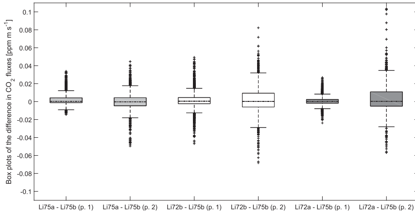
FIG. 6. Boxplots of the difference in measured CO 2 flux between the Li75b instrument and the other three instruments for period 1 (p.1) and period 2 (p.2). In period 2 a Nafion dryer was mounted on one of the Li-7200 instruments (Li-72b). The light gray boxes show the comparison of the two Li-7500 instruments. The white boxes show the comparison of the Li-7200 instrument with a Nafion dryer installed during period 2. The dark gray boxes show the comparison of the Li-7200 instrument without a Nafion dryer (Li72a). The median value is marked (dash–dotted line), and the boxes mark the 25th and 75th percentiles. Outliers are drawn as plus (+) signs if they are larger than Q3 + 1.5(Q3 – Q1) or smaller than Q1 – 1.5 (Q3 – Q1), which define the whiskers of the data. Here Q1 and Q3 are the 25th and 75th percentiles, respectively.
