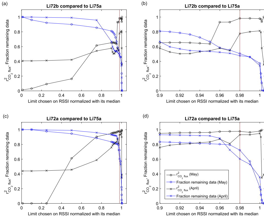
FIG. A2. The squared correlation coefficient for the CO 2 flux (black) and the fraction of remaining data (blue) are shown as a function of different threshold limits for RSSI values normalized by the median RSSI value (RSSI/RSSI). Here the median is taken as the median of the measurement period. The result for the (a) Li-Cor 75a and Li-Cor 72b and the (c) Li-Cor 75a and Li-Cor 72a. (b),(d) Zoomed-in views on the range 0.90–1.01. Data from April 2015 (lines with crosses) and May 2015 (lines with circles). The threshold limit RSSI/RSSI = 0.98 is indicated (vertical red line).
