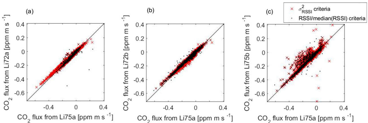
FIG. A3. The measured CO 2 flux from Li-Cor 7500a (both April and May data are included) is compared to the measured fluxes from (a) Li-Cor 7200a, (b) Li-Cor 7200b, and (c) Li-Cor 7500b. Data for the chosen threshold limit \sigma_{RSSI}^2 < 0.001 (red crosses) and other selection criteria RSSI/median(RSSI) > 0.98 are denoted (black dots).
