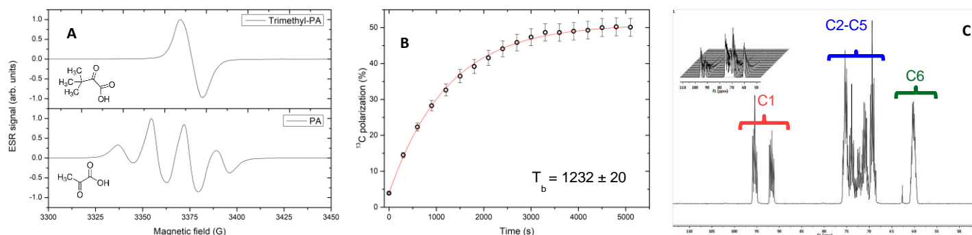
Figure 1A. X-band ESR spectra of UV-irradiated Tri-PA (top) and UV irradiated PA (bottom) at 77 K. B Carbon DNP buildup measured shining microwaves at a frequency of 188.18 GHz with a 25 MHz/1 kHz modulation. C After dissolution 13 C spectrum of glucose at room temperature in a Varian 400 MHz high resolution NMR spectrometer (C).
