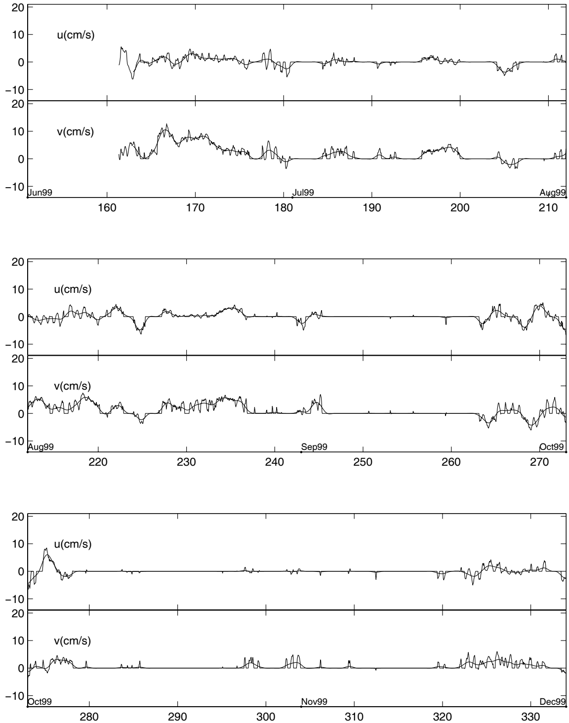
Figure 7: M1-3 Hourly and 40 HRLP Velocities
