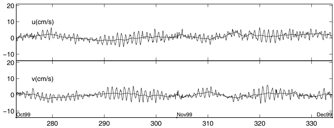
Figure 14: M4-3n Hourly and 40 HRLP Velocities
