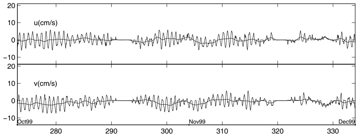
Figure 5: M1-1 Hourly and 40 HRLP Velocities
