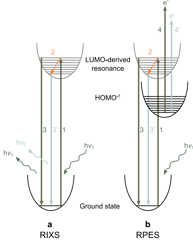
FIG. 1. Schematic of the electronic transitions in the presence and absence of vibronic coupling in a simplified Franck-Condon picture of a) RIXS and b) RPES. Transition 1 is the x-ray absorption event from the N 1s core level in the ground state to a specific vibrational state of the LUMO-derived resonance. Transition 3 is the elastic participator event which leads to an elastic photon ( h\nu_1 ) in RIXS and the emission of an electron (transition 4) in RPES. Transition 2 represents the dissipation of vibrational energy within the core hole lifetime leading to the inelastic participator decay shown by transition 3'. In RIXS this leads to the emission of a photon ( h\nu_2 ) of lower energy (inelastic scattering) and in RPES to the emission of an electron with a lower kinetic energy (transition 4'). While not relevant to the present discussion, it is also possible to end up in a state other than the ground state in RIXS and RPES (omitted for clarity).
