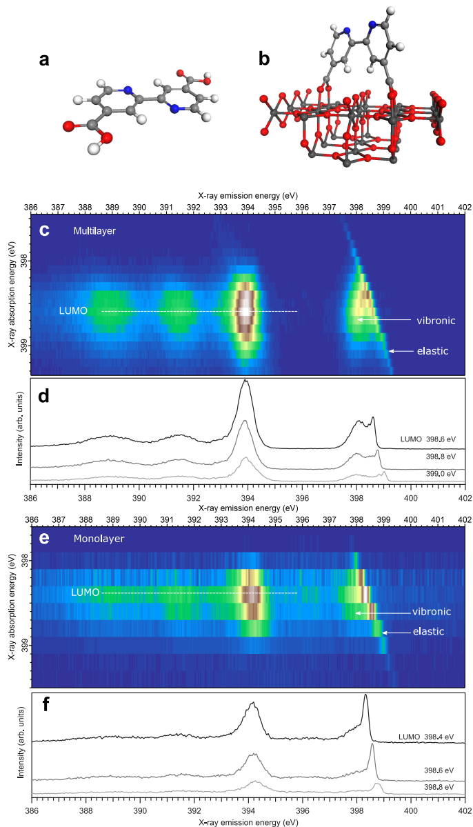
FIG. 2. Molecular structure of a) an isolated bi-isonicotinic acid molecule an b) bi-isonicotinic acid chemisorbed in a 2M-bidentate configuration on the rutile \text{TiO}_2(110) single crystal surface mediated through the deprotonated carboxyl groups. N 1s RIXS maps for c) physisorbed bi-isonicotinic acid multilayer and e) chemisorbed monolayer on the rutile \text{TiO}_2(110) single crystal surface. Single energy RIXS spectra extracted from the RIXS maps at the specified excitation energies for the d) multilayer and f) monolayer. The experimental data is a subset of the data from our previously published RIXS results, rescaled to focus on the participator region of the LUMO-derived resonance. 14
