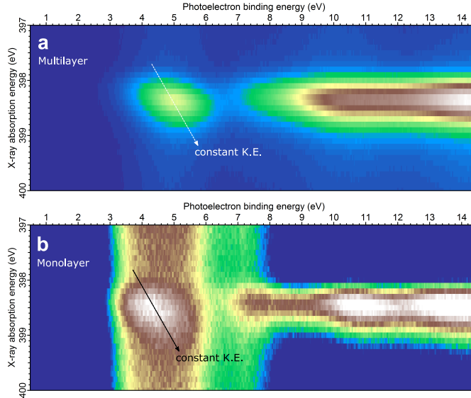
FIG. 3. N 1s RPES maps for a) a physisorbed bi-isonicotinic acid multilayer and b) the chemisorbed monolayer on the rutile \text{TiO}_2(110) single crystal surface. In both spectra a line of constant kinetic energy is added as a guide to show that the participator resonant photoemission signal from the LUMO-Core-HOMO decay channel (see figure 1b) tracks with constant kinetic energy due to vibronic coupling.
