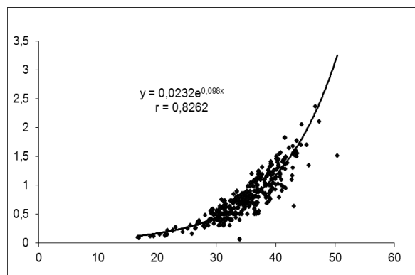
Figure 1: The total length–weight relationships of A.anatolicus from the Lake Eğirdir (♀- ♂)
