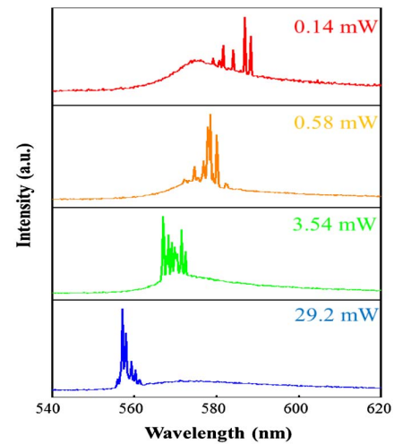
Fig. 11. Stabilized wavelength of RLs changes with varying NIR irradiation power.
