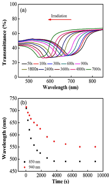
Fig. 9. (a) Transmission spectra of CLC as a function of irradiation time of 940-nm NIR. (b) Bragg wavelength as a function of NIR irradiation time. (■) 850-nm NIR irradiation on the sample; (●) 940-nm NIR irradiation on the sample.)
