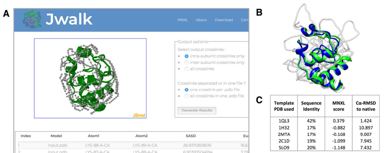
Figure 1 [(A). Partial screenshot of the Jwalk result page with PDB id. 1HRC shown. (B) The models of the test-case superposed in grey, with the best scoring model based on 1QL3 (blue) and the native 1HRC (green). (C) Results table showing MNXL is able to select the lowest C \alpha -RMSD
