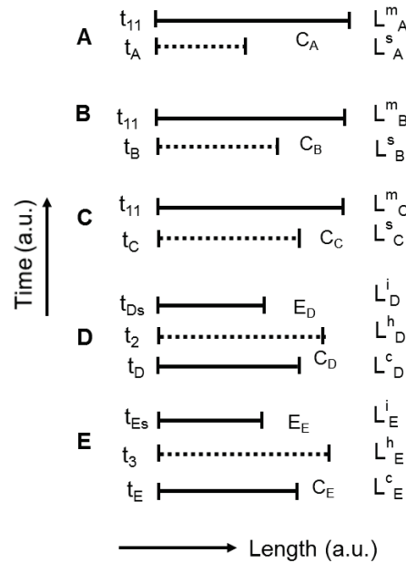
FIGURE 3. The one-dimensional representation of the change of dimension with time during heating and cooling process where the notations for time are taken from the Figure 2.
