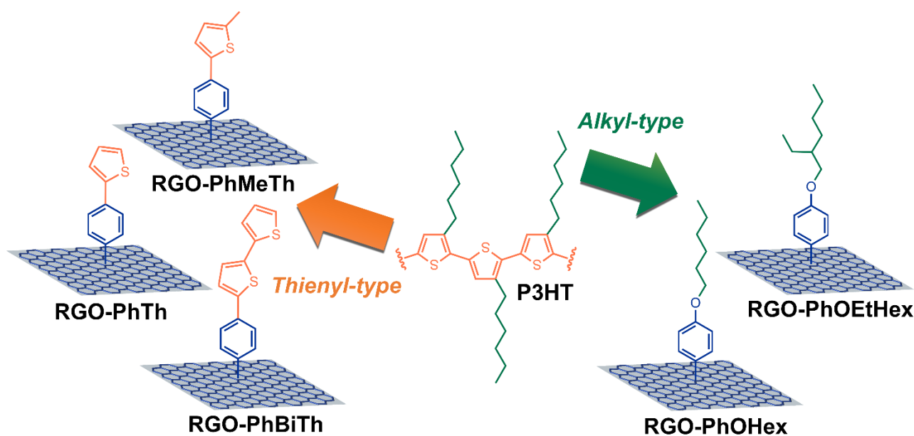
35 Figure 1. Schematic illustration of the five types of functionalized-RGO species reported in this work, highlighting the 36 similarity relationships existing among the organic substituents covalently bound to RGO and the P3HT structure.
