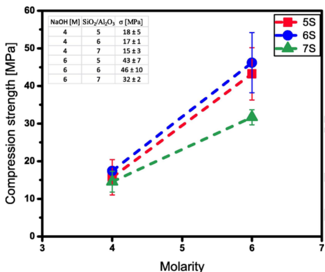
Fig. 3. Compressive strength average results as function of NaOH solution molarity and SiO 2 /Al 2 O 3 molar ratio.
