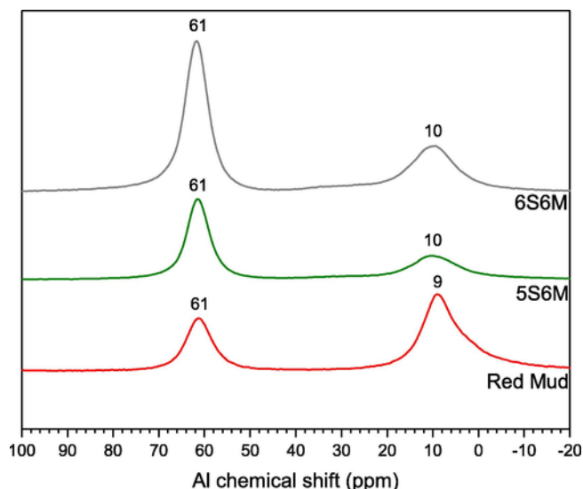
Fig. 2. 27 Al MAS NMR spectra of raw materials and geopolymers activated with 6 M NaOH solution.
