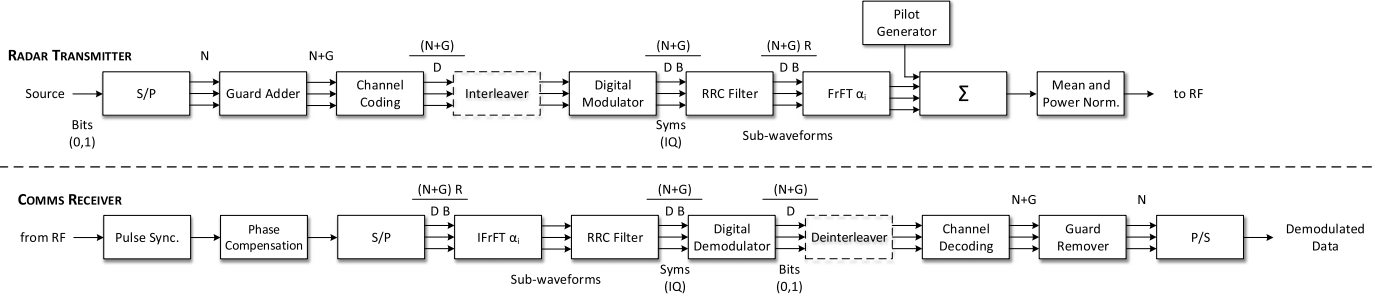
Fig. 2. Block diagram of (top) the FrFT Radar Transmitter, in charge of the waveform generation, and (bottom) the FrFT Communication Receiver, whose task is the demodulation of the received pulses.
