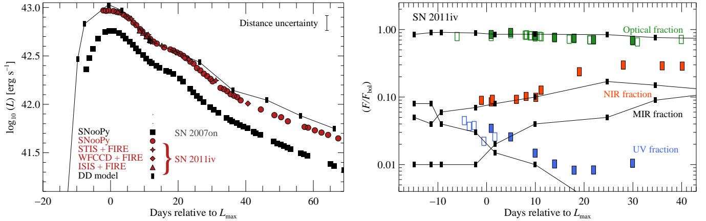
Fig. 11. Left: bolometric light curves of SN 2007on (black) and SN 2011iv (red) constructed from observations constraining the flux extending from uvm2 to the H band ( \sim 2250\text{--}18\,800\text{ \AA} ; UVOIR). Complementing the majority of SN 2011iv measurements are a handful of additional bolometric points covering the wavelength range extending from the UV ( 1620\text{ \AA} ) to K_s ( 24\,900\text{ \AA} ). The error bar on the bolometric luminosity is presented in the top right of the plot, and assumes an error in the adopted distance modulus of \pm 0.2 mag. Also shown is the bolometric light curve (line) of model 5p0z22.18b presented in Sect. 6.2. Right: UV (blue), optical (green), and NIR (red) flux fractions of the total bolometric light curve of SN 2011iv computed from observed spectroscopy. The open green symbols illustrate reduced optical flux fractions from 3480\text{ \AA} to 8630\text{ \AA} , while the solid green symbols represent the full range from the atmospheric cutoff at 3050\text{ \AA} to 8630\text{ \AA} . The UV fraction extends from either 1620\text{ \AA} (STIS, solid blue symbols) or 1900\text{ \AA} (UVOT, open blue symbols) to 3050\text{ \AA} , and the NIR fraction extends from 9000\text{ \AA} to 24\,900\text{ \AA} . Shown as connected filled squares is the fraction of flux distributed among the different wavelength regimes for model 5p0z22.18b. This includes the predicted MIR fraction ( 24\,900\text{ \AA} to 1\,000\,000\text{ \AA} ), which drives the difference between the observed and modelled UVOIR light curves beginning around a month past maximum brightness.
