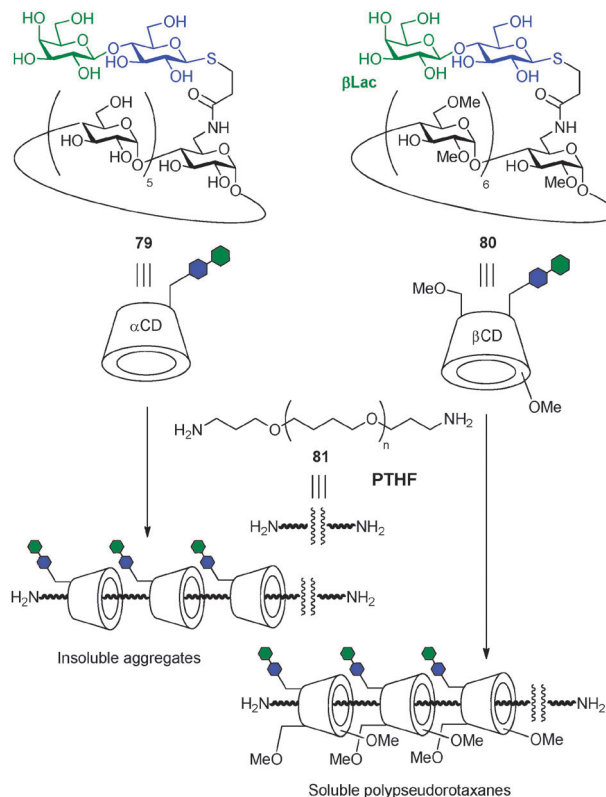
Scheme 34 Schematic representation of multilactosylated pseudorotaxanes assembling from monolactosylated CD conjugates. 128
