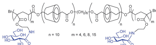
Fig. 9 Glycopolymer-pseudopolyrotaxane biohybrids. 133
