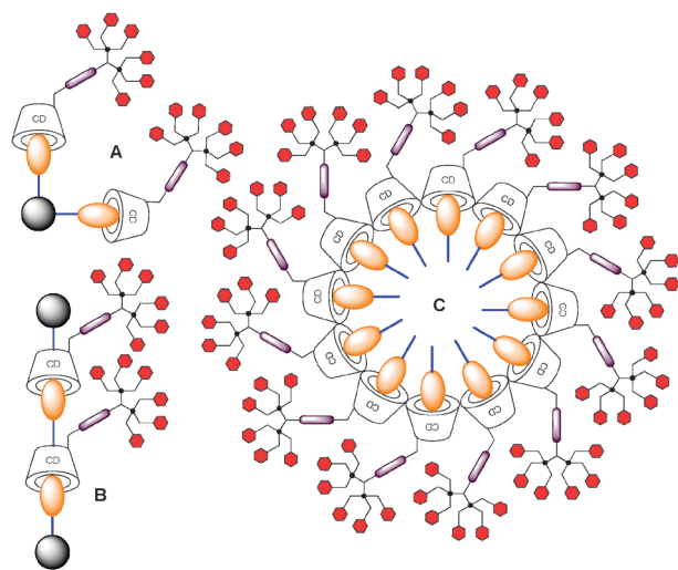
Fig. 2 Examples of self-assembled multivalent architectures from CD–glycoligand (in red) conjugates promoted by either a guest partner or a functional moiety (in orange): (A) multiprotic inclusion complex; (B) polyrotaxane; (C) micelle, vesicle or nanocomplex.
