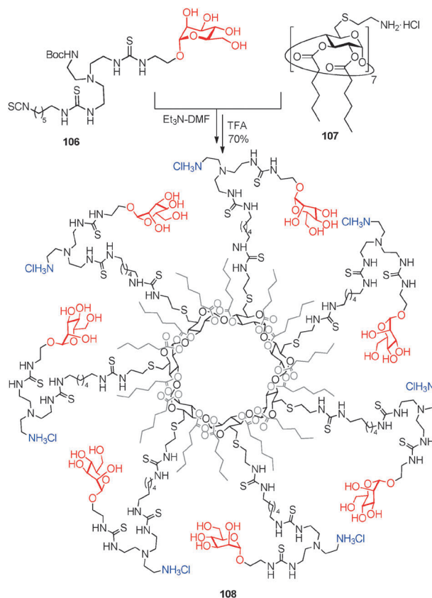
Scheme 44 Synthesis of the \alpha Man-pGaCD gene vector prototype proposed by García Fernández and co-workers. 167
