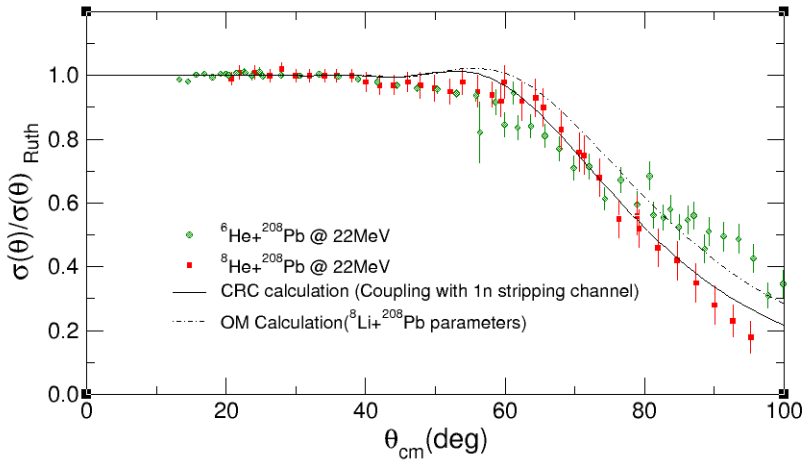
Fig. 1. Angular distribution of the elastic cross section for the systems {}^8\text{He}+{}^{208}\text{Pb} and {}^6\text{He}+{}^{208}\text{Pb} , both at E_{\text{lab}} = 22 MeV. See the text for details.
