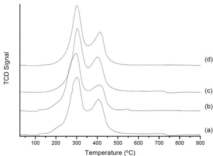
Figure 2. Thermal programmed reduction curves of \text{MnO}_x -based catalysts: (a) \text{MnO}_x ; (b) \text{Ce/MnO}_x ; (c) \text{Au/MnO}_x and (d) \text{Au/Ce/MnO}_x .
