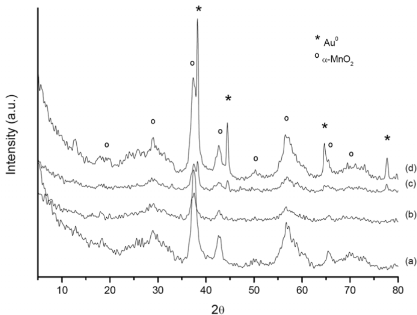
Figure 1. X-ray diagram of \text{MnO}_x -based catalysts: (a) \text{MnO}_x ; (b) \text{Ce/MnO}_x ; (c) \text{Au/Ce/MnO}_x and (d) \text{Au/MnO}_x .
