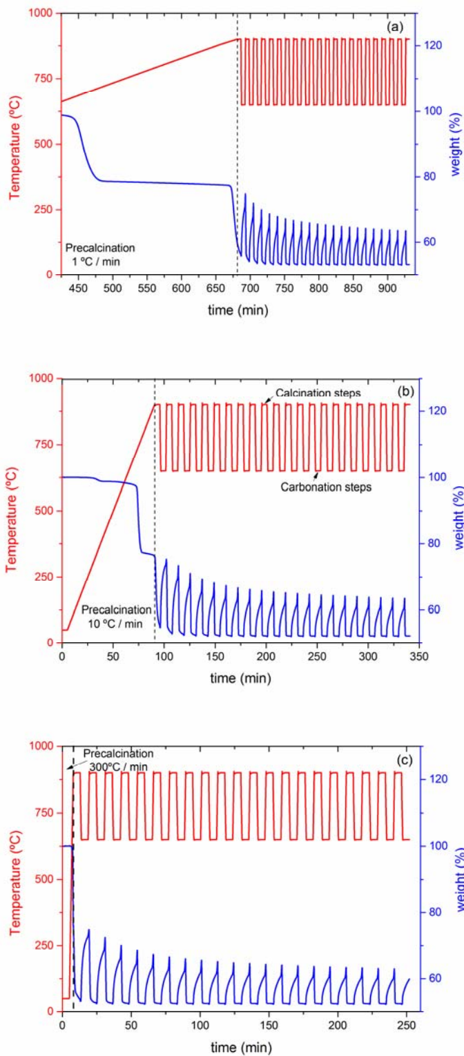
Figure 2. Time evolution of weight % and temperature during multicycle carbonation/calcination of dolomite after precalcination at different heating rates: (a) 1°C/min; (b) 10°C/min; (c) 300°C/min. Carbonations at 650 °C in 15% CO 2 / 85% air (vol/vol) for 5 min and calcinations at 900 °C in 70% CO 2 / 30% air (vol/vol) for 5 min.
