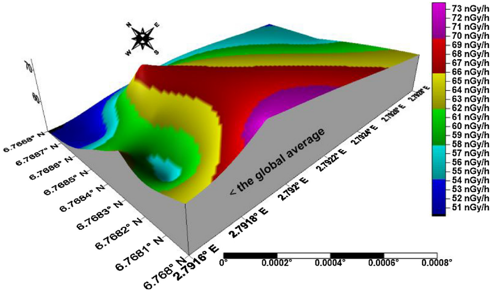
Fig. 5. Isodose map of kaolin deposits in Ifonyintedo (upper axis).
