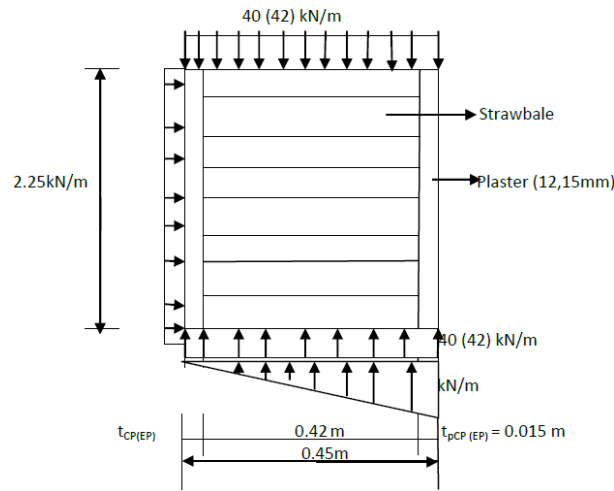
Fig. 1 Cross section of cement (earth) plastered strawbale wall
