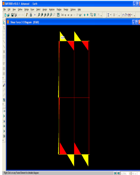
Fig. 6 Shear force diagram of earth plastered typha strawbale wall
