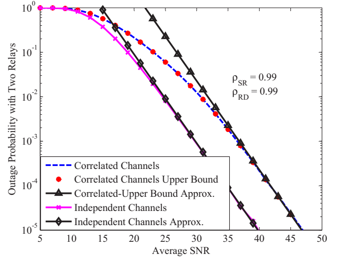
Fig. 1. Outage probability of two-relay systems versus average SNR.
