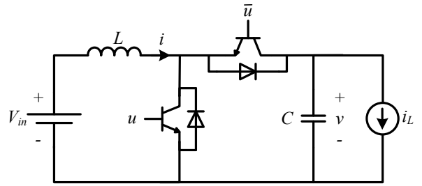
Fig. 1. Bidirectional dc/dc power converter
