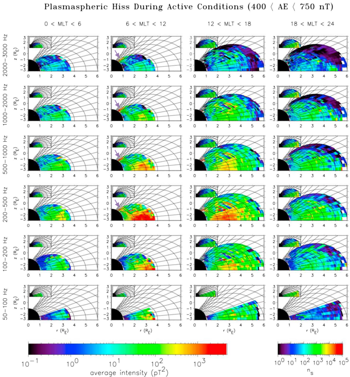
Figure 7. Global maps of the average wave intensity of plasmaspheric hiss in the meridional plane during active conditions, 400 < AE < 750 nT, for, from bottom to top, increasing wave frequency and for, from left to right, increasing magnetic local time. To aid visualization of the data, dipole field lines and lines of constant magnetic latitude are included on the plot. The average intensities are shown in the large panels and the corresponding sampling distributions in the small panels. In the prenoon sector the purple arrows point to the location of the high-latitude plasmaspheric hiss.
