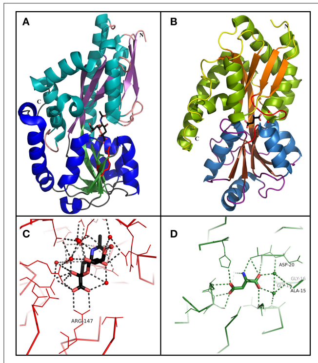
FIGURE 3 | Comparison between TRAP and TTT SBP crystal structures. (A) Overall structure of SiaP, a sialic acid binding SBP from the TRAP family in H. influenzae (PDB 3B50). Domain 1 is represented in cyan ( \alpha -helix) and purple ( \beta -sheet), and domain 2 is represented in blue ( \alpha -helix) and green ( \beta -sheet). A sialic acid molecule is shown in the binding pocket. Arg147, important to perform a salt bridge with the carboxylic group of the substrate in most SiaP homologs is shown in red. (B) Overall structure of BugD, a aspartate binding SBP from the TTT family in B. pertussis (PDB 2F5X). Domain 1 is represented in green ( \alpha -helix) and orange ( \beta -sheet), and domain 2 is represented in blue ( \alpha -helix) and brown ( \beta -sheet). An aspartate molecule is shown in the binding pocket. Two loops, between \beta 1 and \alpha 1 and between \beta 7 and \alpha 6 , are involved in the conserved coordination of two water molecules, which bridge hydrogen bonds with the proximal carboxylic group in the substrate. These loops and waters are shown in red. (C) Binding pocket of SiaP, showing the coordination of the sialic acid molecule. Arg147 perform a salt bridge with the carboxylic group in the substrate. The remaining of the molecule is coordinated by hydrogen bonds and water molecules which are variable inside the TRAP family. (D) Binding pocket of BugD, showing the coordination of the aspartate molecule. The residues Ala-15, gly-16, gly-17, and Asp-20 participate in the loop between \beta 1 and \alpha 1 , coordinating two water molecules which bridge hydrogen bonds with the proximal carboxylic group in the substrate. This coordination is very conserved among the TTT family. The remaining substrate coordination occur through non-conserved hydrogen bonds and water bridging.
