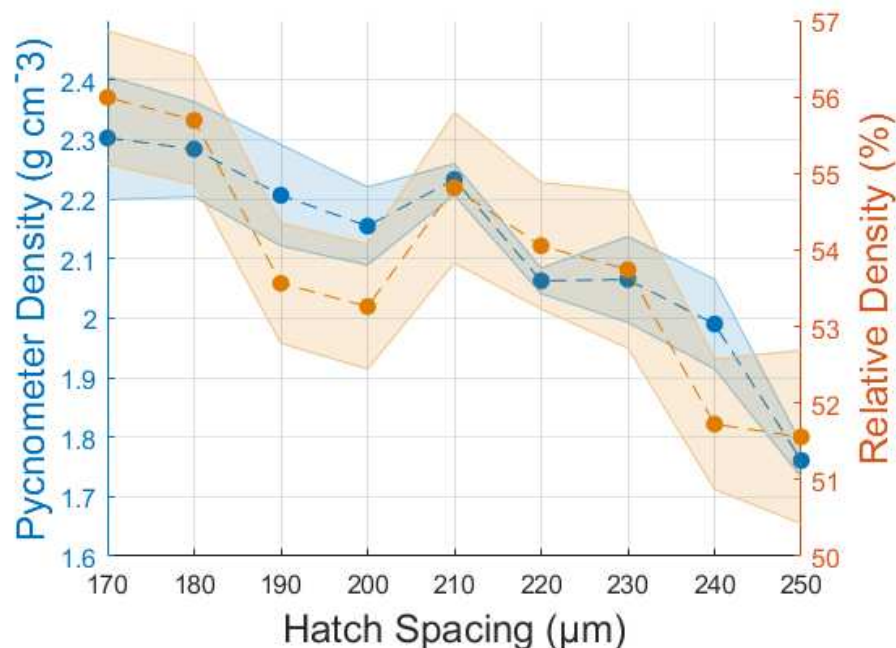
Figure 10 – Comparison of measured 3D printed samples densities as measured using pycnometry and from the relative porosity values obtained by SEM analysis. The shaded areas represent the standard error.
