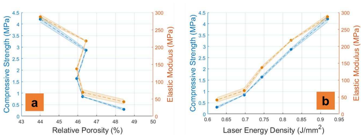
Figure 15 – Influence of relative porosity (%) and energy density on the compressive strength and elastic modulus of additively manufactured parts from lunar regolith simulant. The shaded areas represent the standard error.
