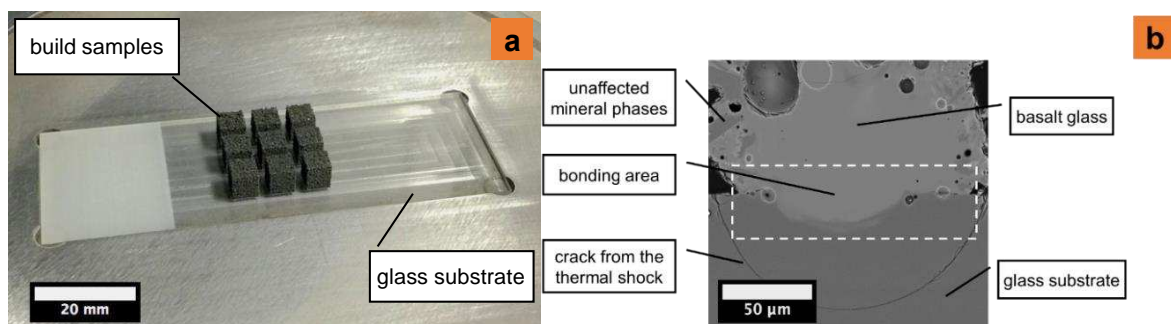
Figure 3 – (a) Additively manufactured 5 mm cuboid samples, built on a borosilicate glass substrate and (b) bonding between the two glass (basalt-borosilicate) materials after laser processing.
