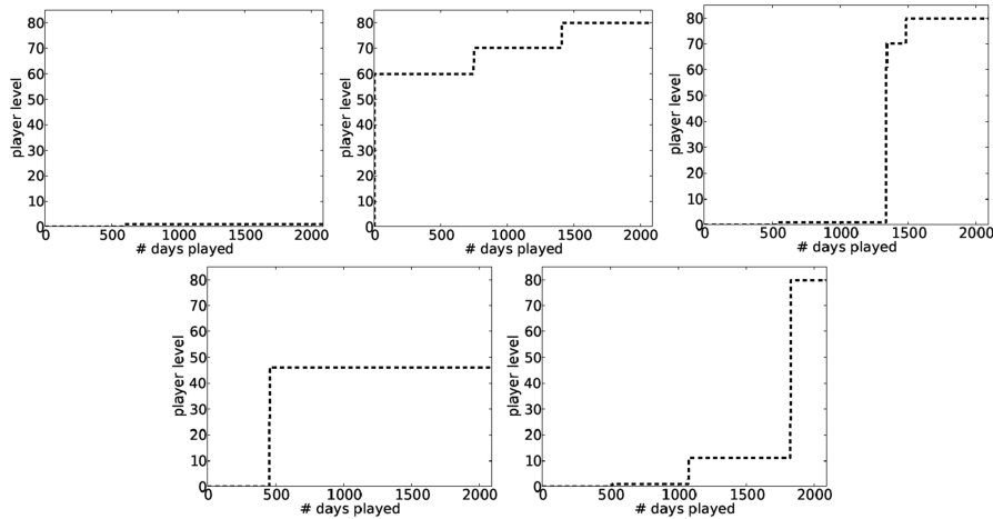
Fig. 12.4 Basis vectors for Archetypal Analysis. These reside on data samples (players in this case). All basis vectors correspond to legal player behavior (e.g. players do not lose levels). Note the straight line segments which map directly to level increases
