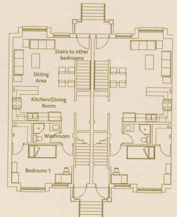
Sample Floor Plan: Townhouse-Style Residence
