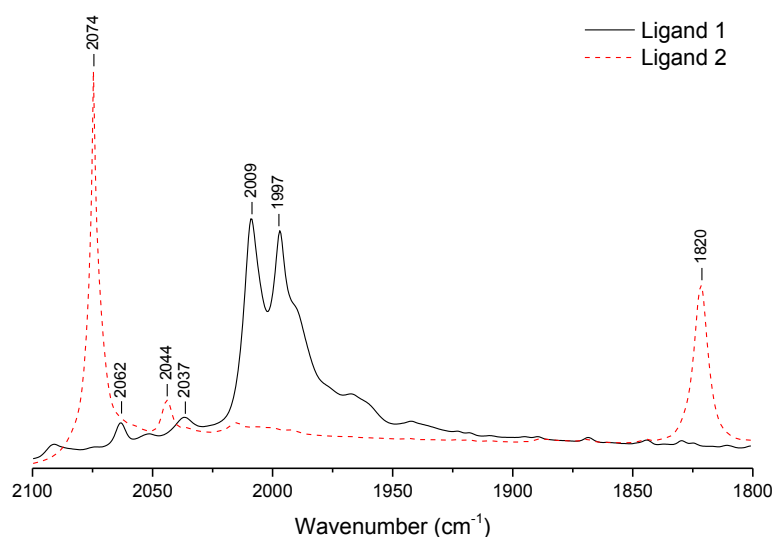
Fig. 3: HPIR spectra of rhodium catalysts from [\text{Rh}(\text{acac})(\text{CO})_2] 70 °C in hexane, under 20 bar syngas (CO:H 2 1:1); from ligand 1 (black) and ligand 2 (red)
