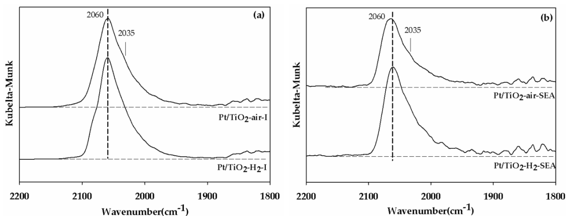
Figure 4. The IR spectra of adsorbed CO on 0.5 wt % Pt/TiO 2 catalysts prepared by: (a) impregnation method and (b) SEA method.
