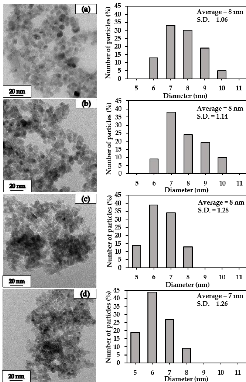
Figure 2. TEM images and size distribution of the Pt/TiO 2 catalysts: (a) Pt/TiO 2 -H 2 -I; (b) Pt/TiO 2 -air-I; (c) Pt/TiO 2 -H 2 -SEA; and (d) Pt/TiO 2 -air-SEA.
