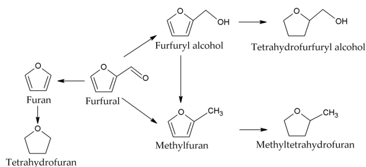
Scheme 2. Simplified reaction pathways in the hydrogenation of FFR.
