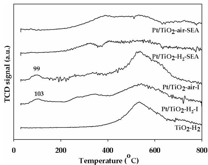
Figure 3. The H 2 -TPR profiles of the Pt/TiO 2 catalysts.
