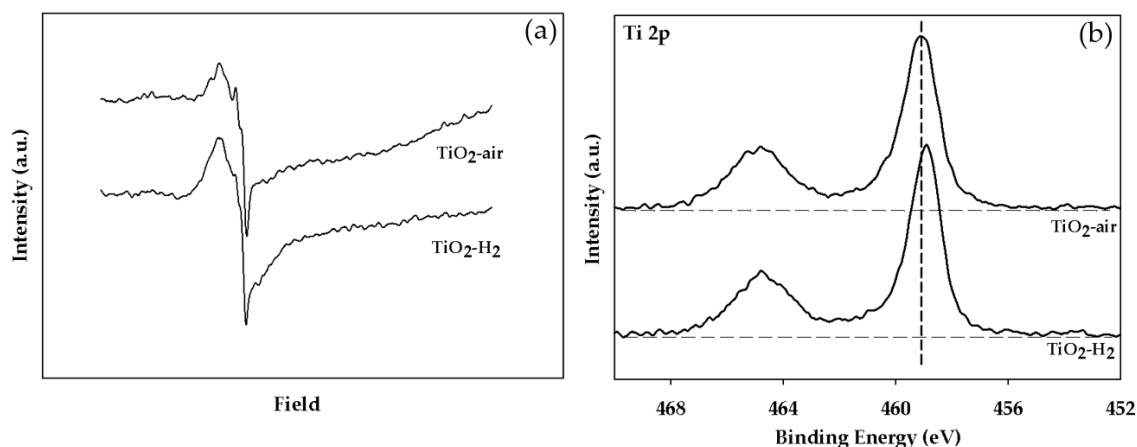
Figure 1. (a) The ESR results of \text{TiO}_2 calcined under \text{H}_2 and air atmosphere at 350 °C and (b) XPS spectra of Ti 2p of \text{TiO}_2 supports.
