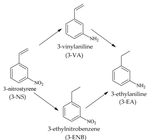
Scheme 1. Simplified reaction pathways in the hydrogenation of 3-NS.
