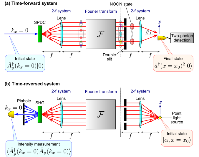
FIG. 2: (Color online) Schematics of (a) time-forward and (b) time-reversed two-photon Young interferometers.
