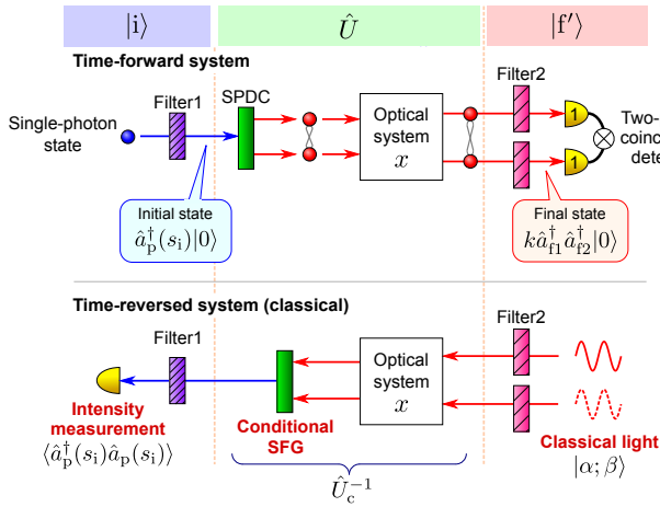
FIG. 8: (Color online) Schematics of general two-photon system in which each of the two photons is detected in different output modes (upper panel) and its classical time-reversed system (lower panel). The time-reversed system can be prepared by the use of a classical optical system in which classical input light, conditional SFG, and intensity measurement are employed.
