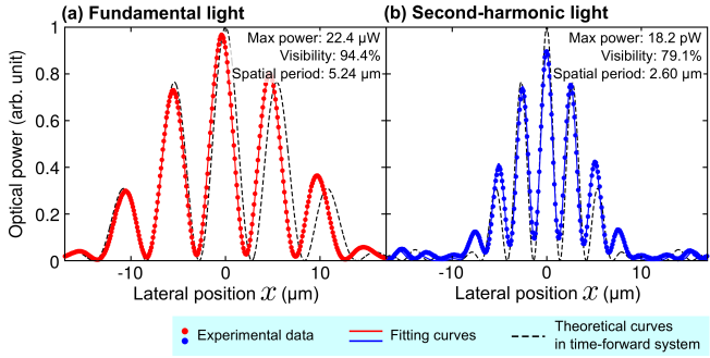
FIG. 4: (Color online) Experimental results of the time-reversed two-photon Young interferometer for fundamental light (a) and second-harmonic light (b). The optical powers in the longitudinal axes are normalized by the measured maximum powers of 22.4 \mu\text{W} (a) and 18.2 pW (b), respectively. The solid curves represent fitting curves; the dashed curves represent the theoretical curves in the time-forward classical and two-photon Young interferometers with the same experimental conditions as this set of experiments.
