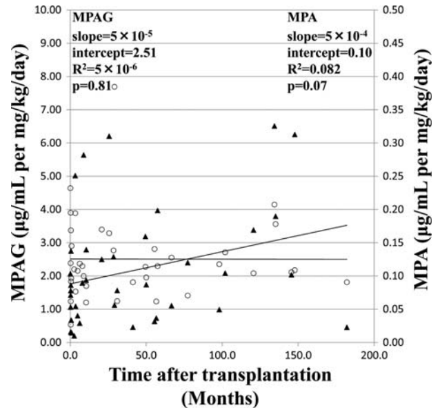
FIGURE 1. MPAG or MPA trough concentrations are not affected by the time after transplantation. Correlation between the time after transplantation and MPAG or MPA. Results are expressed as µg/mL per mg/kg per day. Open circles represent MPAG and solid triangles represent MPA.
